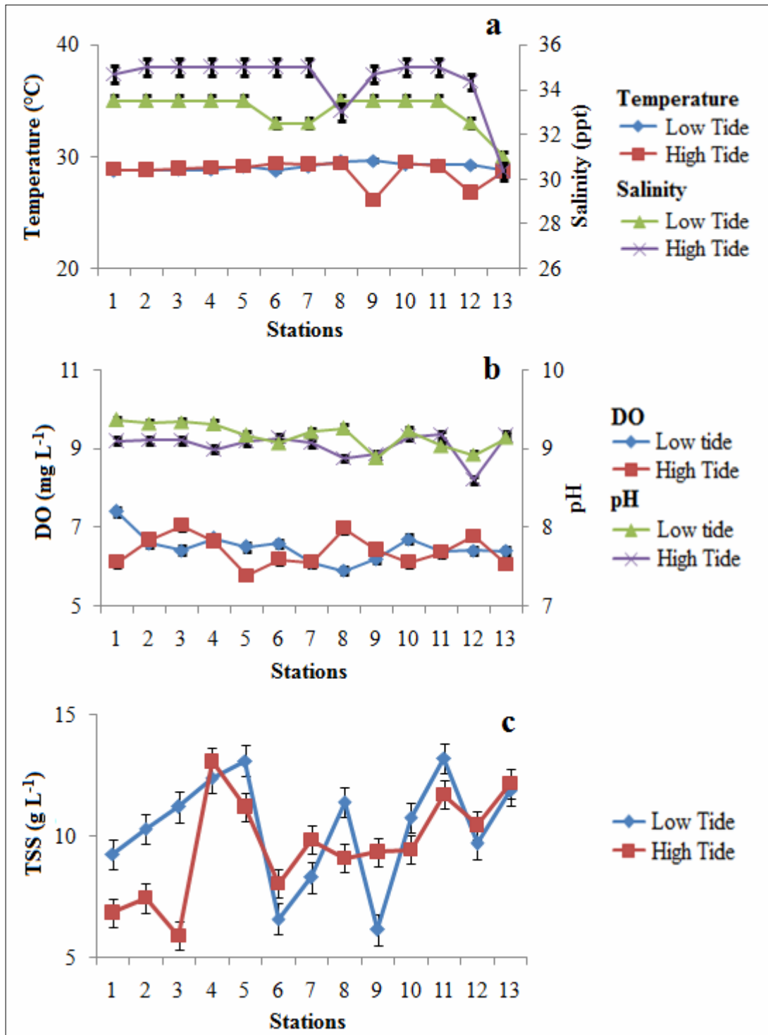
Figure 6. Mean values of (a) water temperature ( ^{\circ}\text{C} ) and salinity (ppt); (b) DO ( \text{mg L}^{-1} ) and pH; (c) TSS ( \text{g L}^{-1} ) in the thirteen sampling stations during low and high tides in Casiguran Sound and Bay, Aurora, Philippines.
